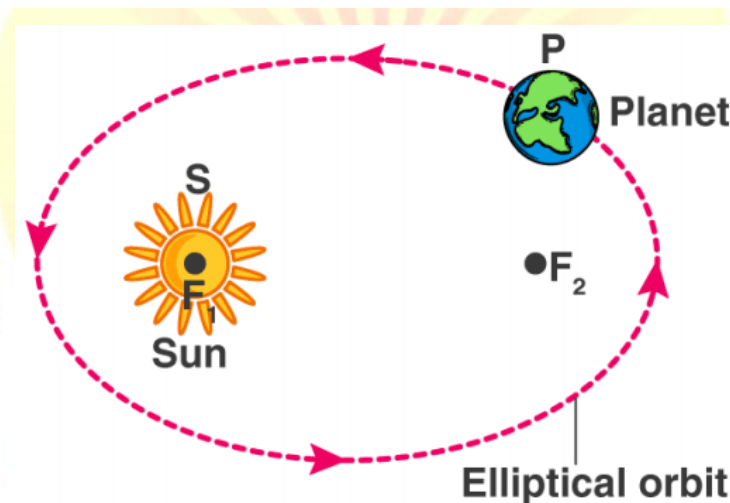
Kepler's First Law
