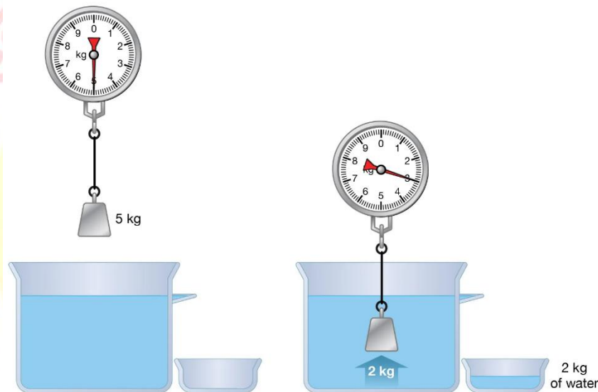
Archimedes' principle
